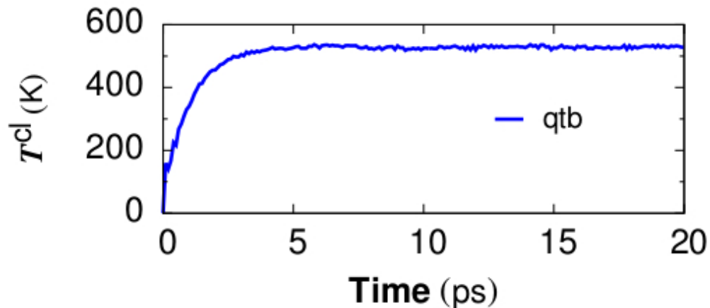
Coupling the Initial State with the QTB T^{\text{qm}} = 300\text{K}
